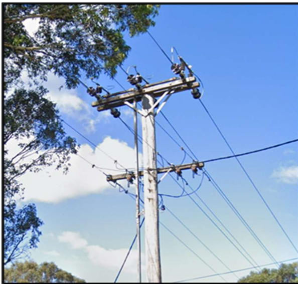
High and low voltage overhead mains
